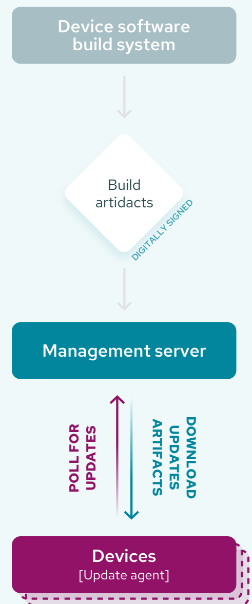
Figure 2: Main components of the over-the-air update system
