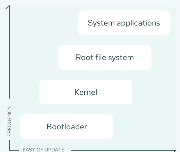
Figure 1: Requirements of an updater
